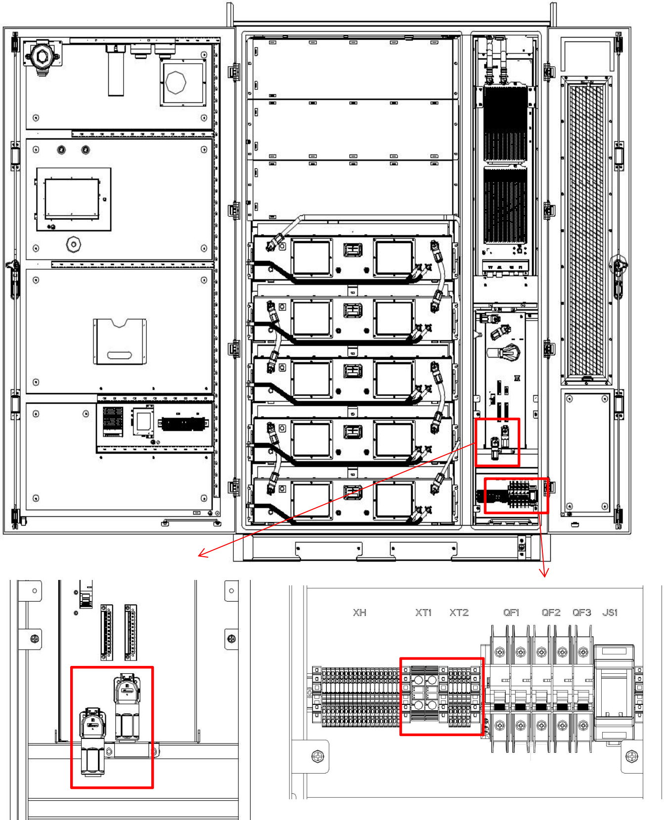
Figure 5.3.4.1 Schematic Diagram of Power Line and Auxiliary Power Supply Line Connection Locations
