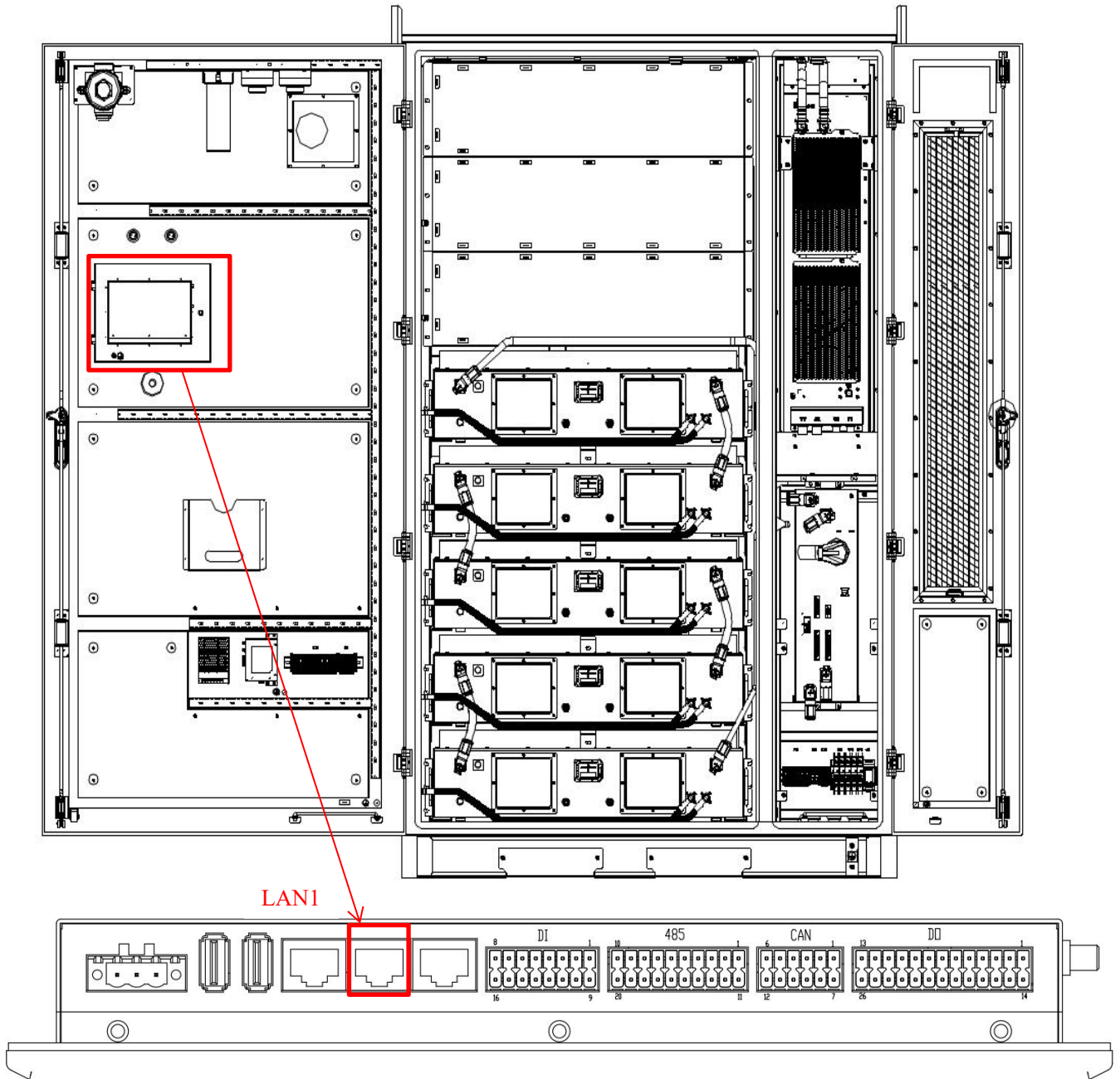
Figure 5.3.5.1 Schematic diagram of the external communication interface of the cabinet
