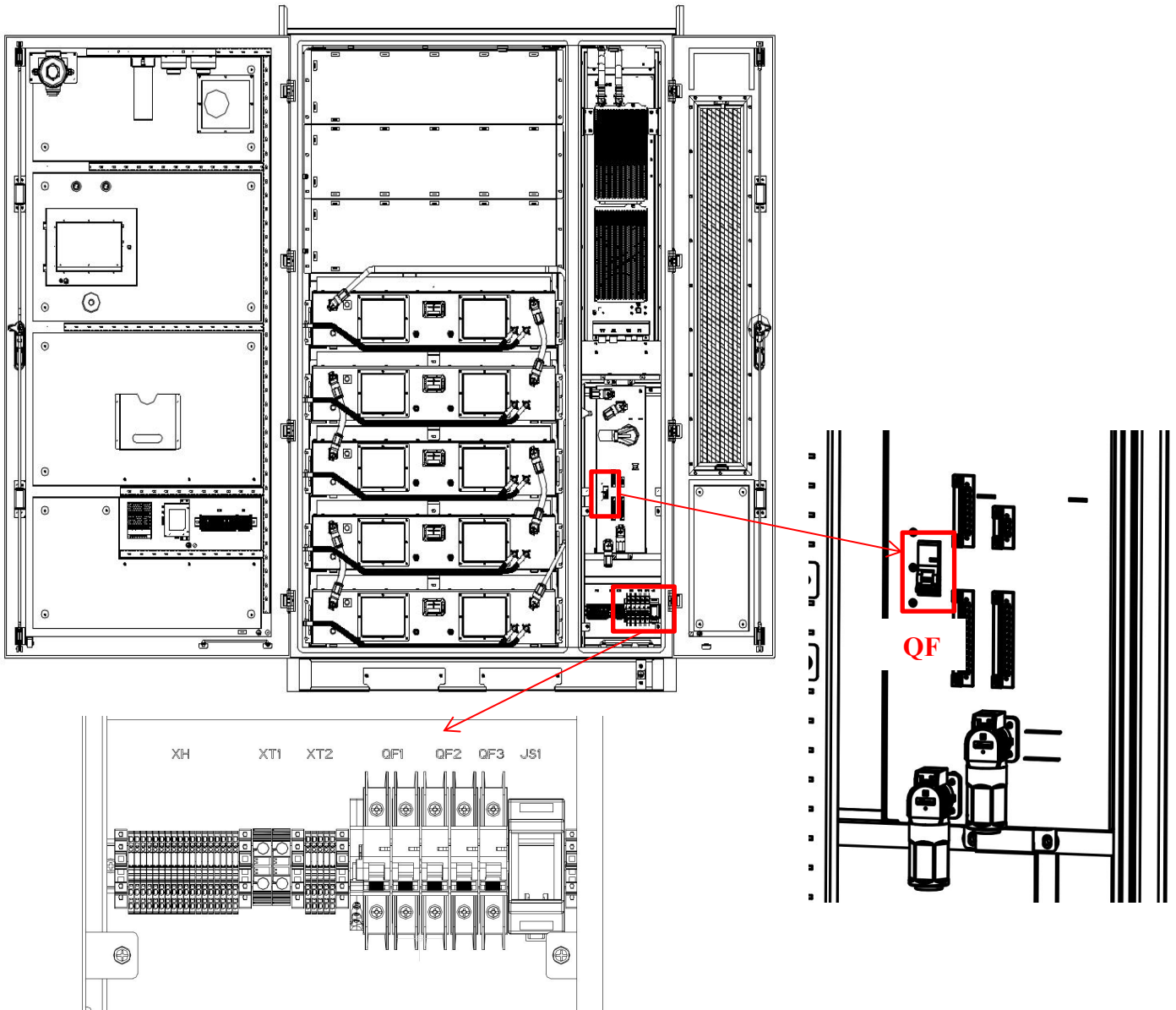
Figure 6.2.2.2 Schematic diagram of the control box
