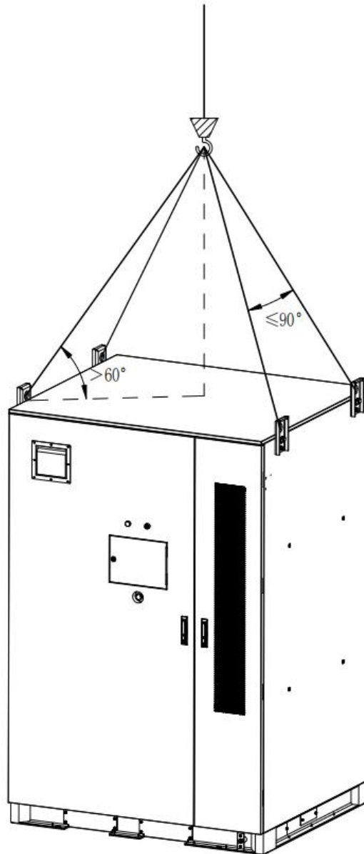
Figure 5.2.3.1 Lifting Schematic
