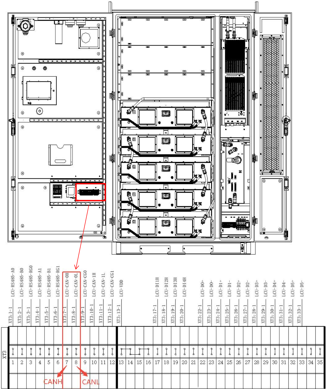
Figure 5.3.5.2 Schematic Diagram of the Cabinet's PCS Communication Interface
