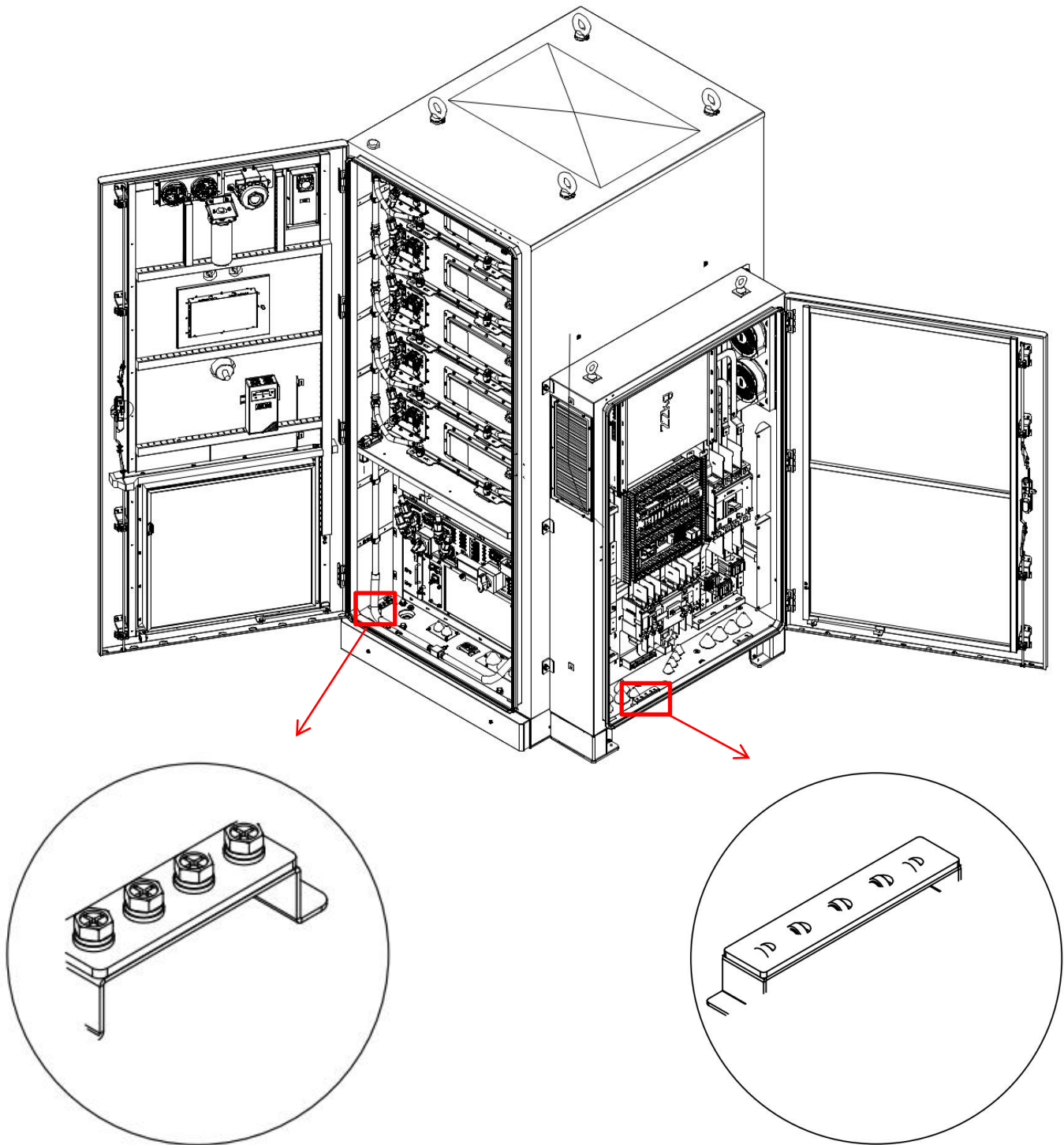
Figure 5.4.3.1 Grounding positions inside the cabinet and inside the STS box
