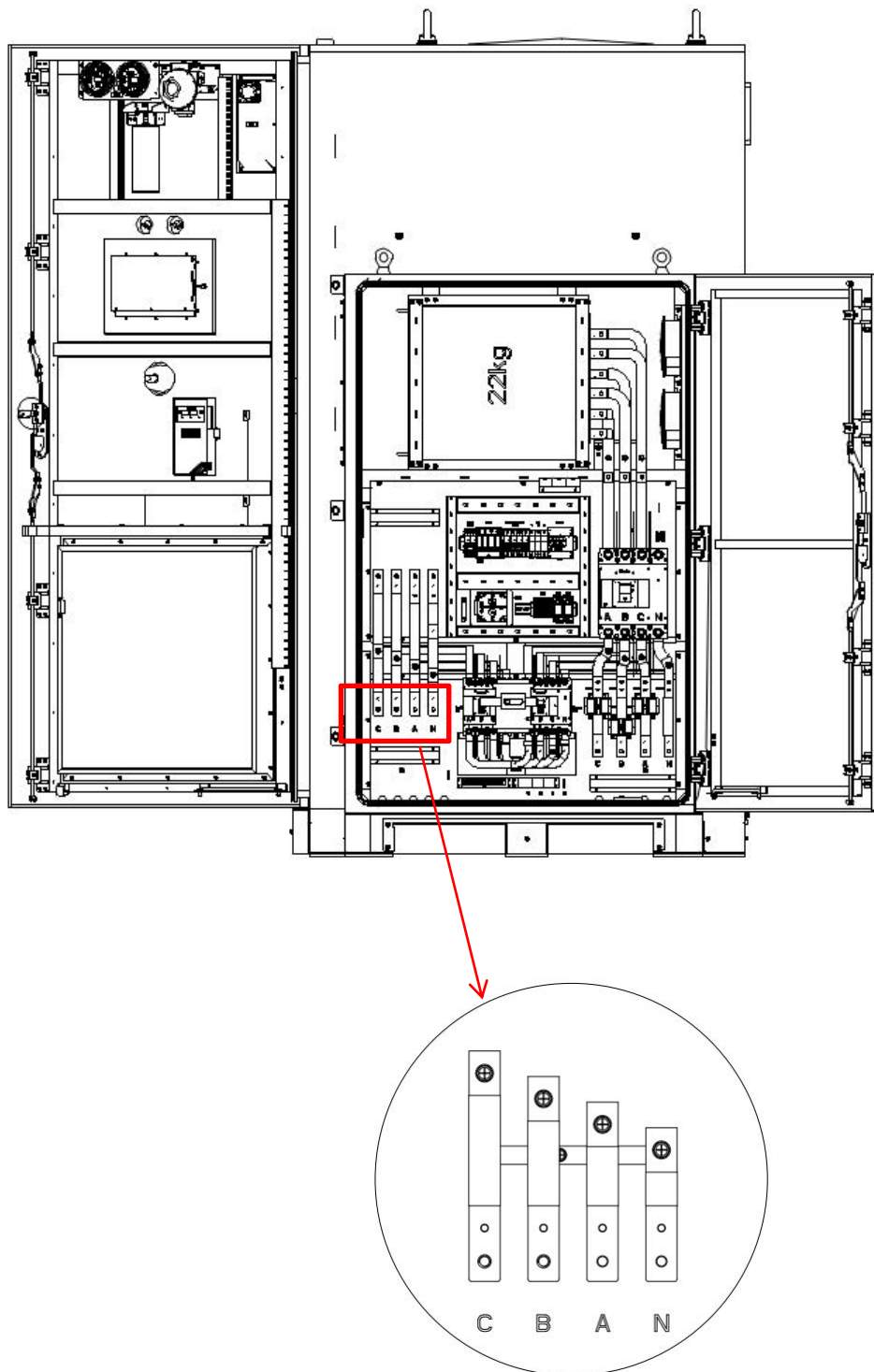
Figure 5.4.3.3 Wiring position of STS box
